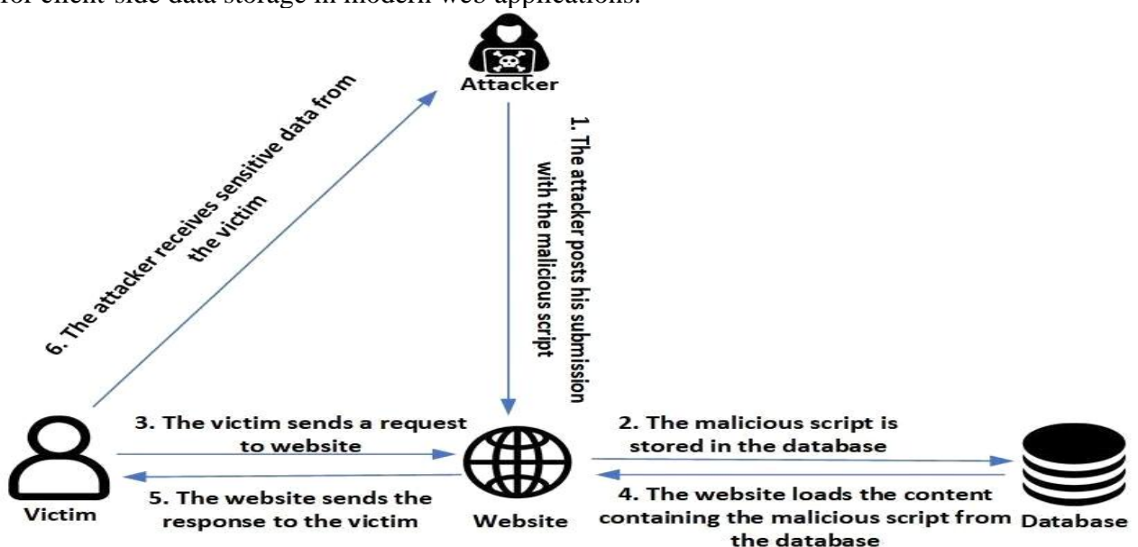
Figure 2 :Process of a stored XSS attack.
