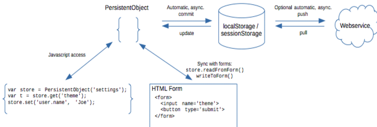
Figure 1 Client-side storage workflow.
